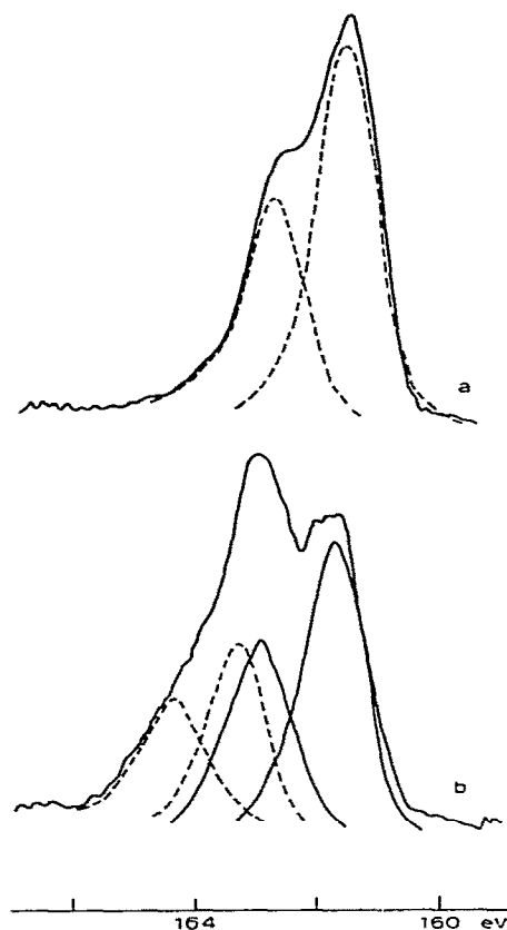
Fig. 2. Sulfur 2 p binding energy spectra of (a) \text{MoO}_2[(\text{SCH}_2\text{CH}_2)_2\text{NCH}_2\text{CH}_2\text{NMe}_2] , and (b) \text{MoO}_2[(\text{SCH}_2\text{CH}_2)_2\text{NCH}_2\text{CH}_2\text{SMe}] . Spectrum (b) has been deconvoluted into two sets of S 2 p 1/2,3/2 spin-orbit doublets. (Reproduced with permission from ref. 35. Copyright by the American Chemical Society.)
