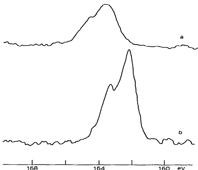
Fig. 1. Sulfur 2 p binding energy spectra of (a) [\text{Pt}(\text{SPh})_2]_n , and (b) cis - \text{Pt}(\text{SPh})_2(\text{CyNC})_2 . (Reproduced with permission from ref. 18. Copyright by the American Chemical Society.)
