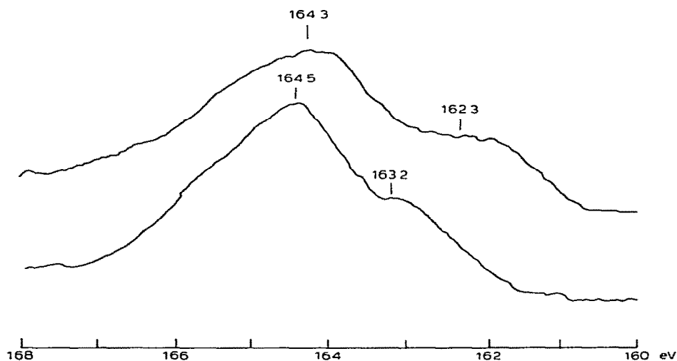
Fig. 3. Sulfur 2 p binding energy spectra of (a) isoperthiocyanic acid, and (b) \text{PtCl}_2(\text{L})_2 . (Reproduced with permission from ref. 60.)
